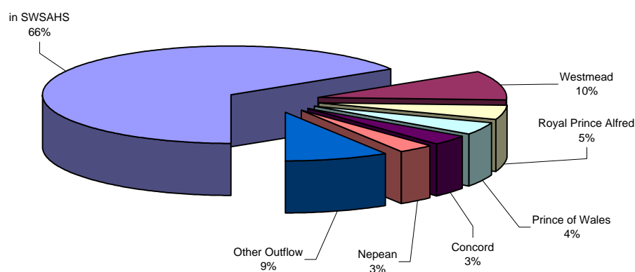
Figure 2.6 Location of Public Sector Treatment for SWSAHS Residents 2002/3: TRACHEOSTOMY (Seps)*
